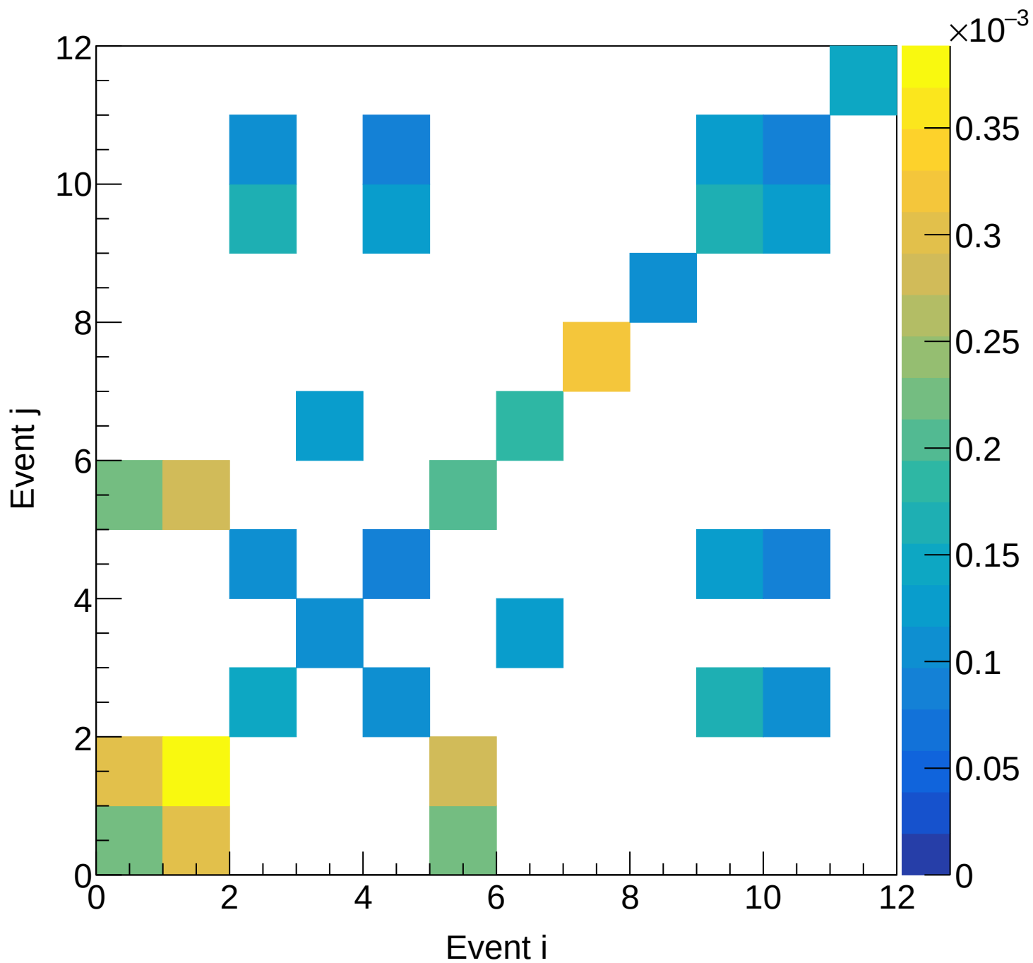
LD2 (total) Covariance | M: [5.4, 5.7) xF: [0.80, 0.85)
