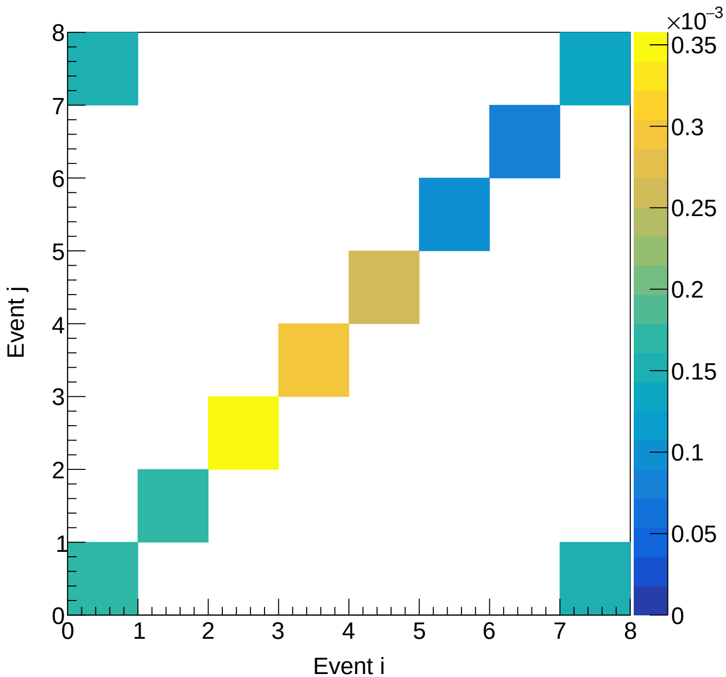
LD2 (total) Covariance | M: [5.7, 6.0] xF: [0.80, 0.85)
