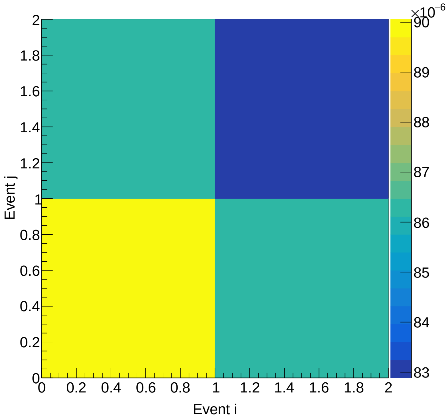
LD2 (total) Covariance | M: [6.0, 6.3] xF: [0.80, 0.85]
