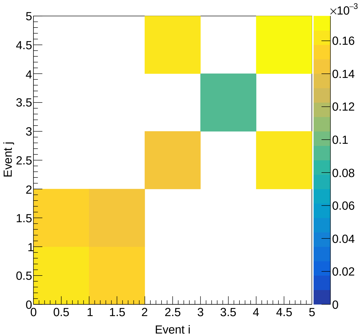
LD2 (total) Covariance | M: [6.3, 6.6) xF: [0.80, 0.85)
