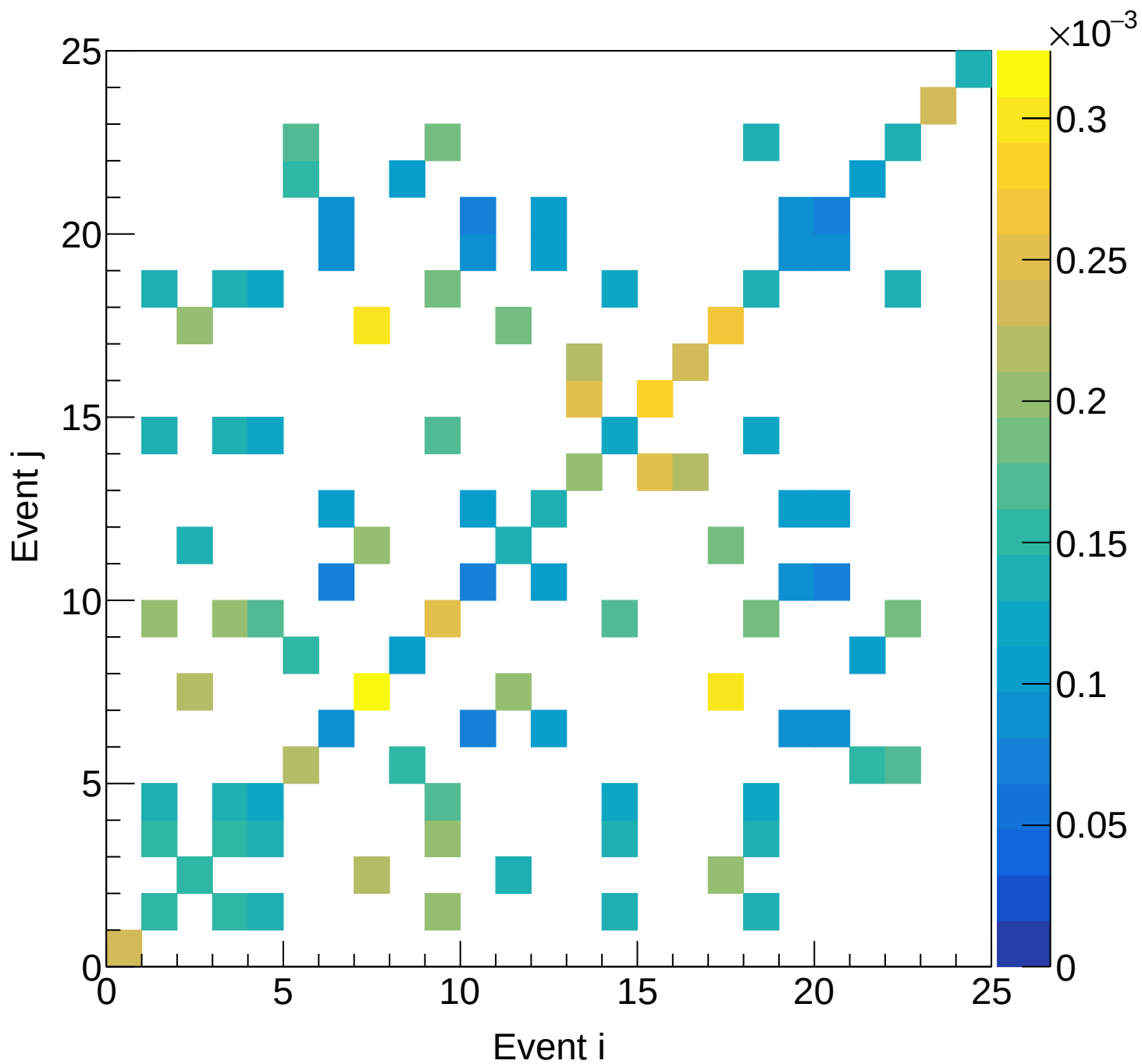
LD2 (total) Covariance | M: [4.2, 4.5) xF: [0.85, 0.90)
