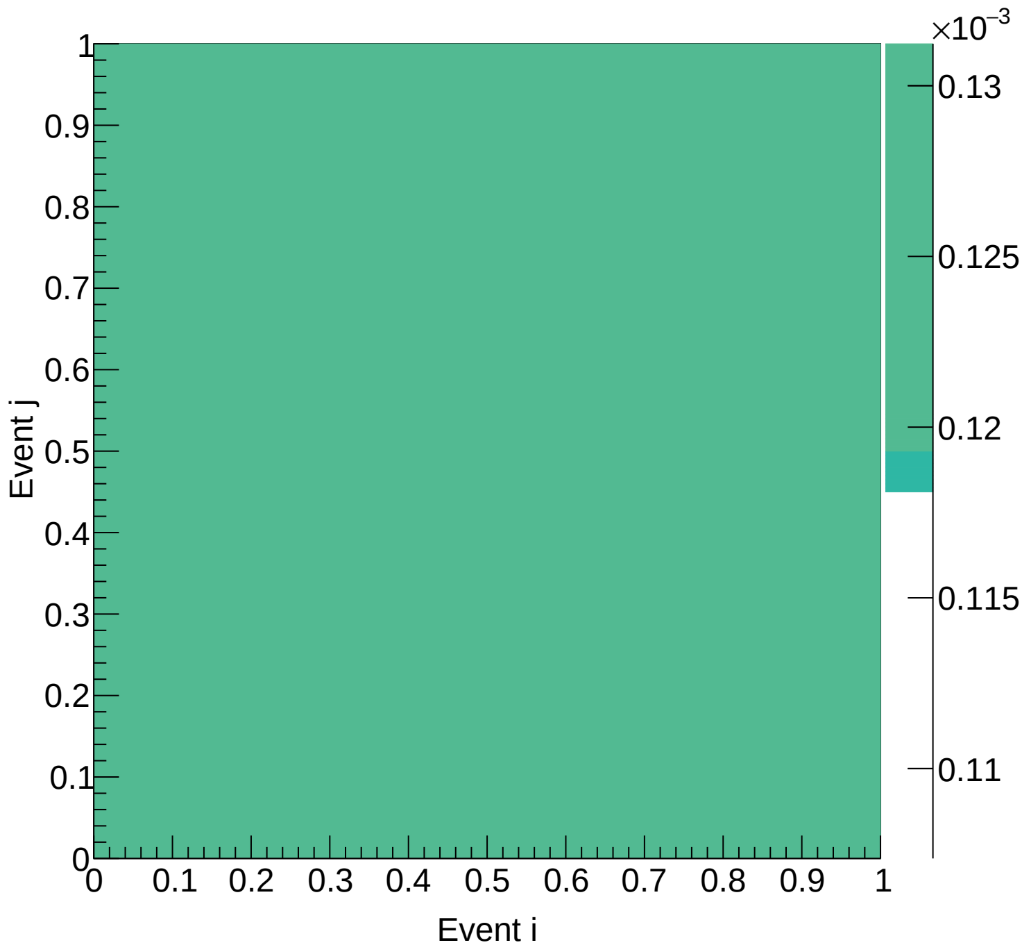
LD2 (total) Covariance | M: [5.7, 6.0) xF: [0.85, 0.90)
