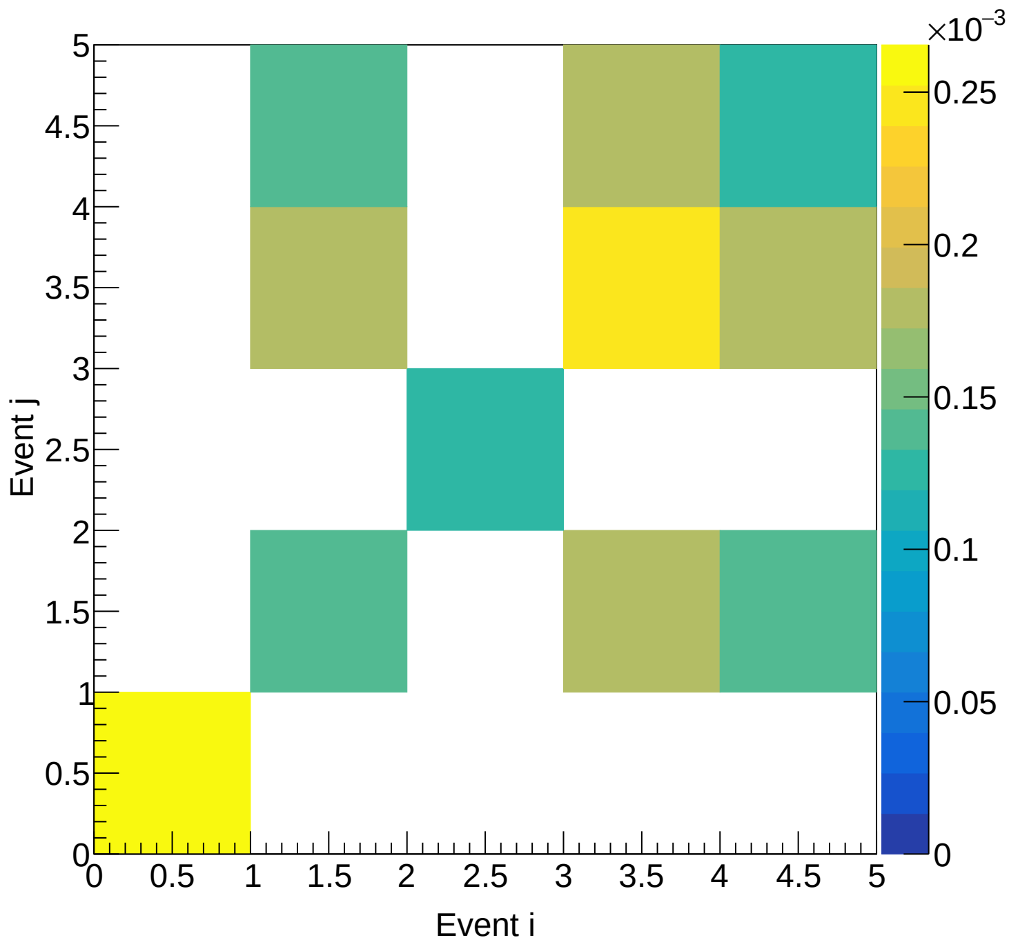
LD2 (total) Covariance | M: [4.2, 4.5) xF: [0.90, 0.95)
