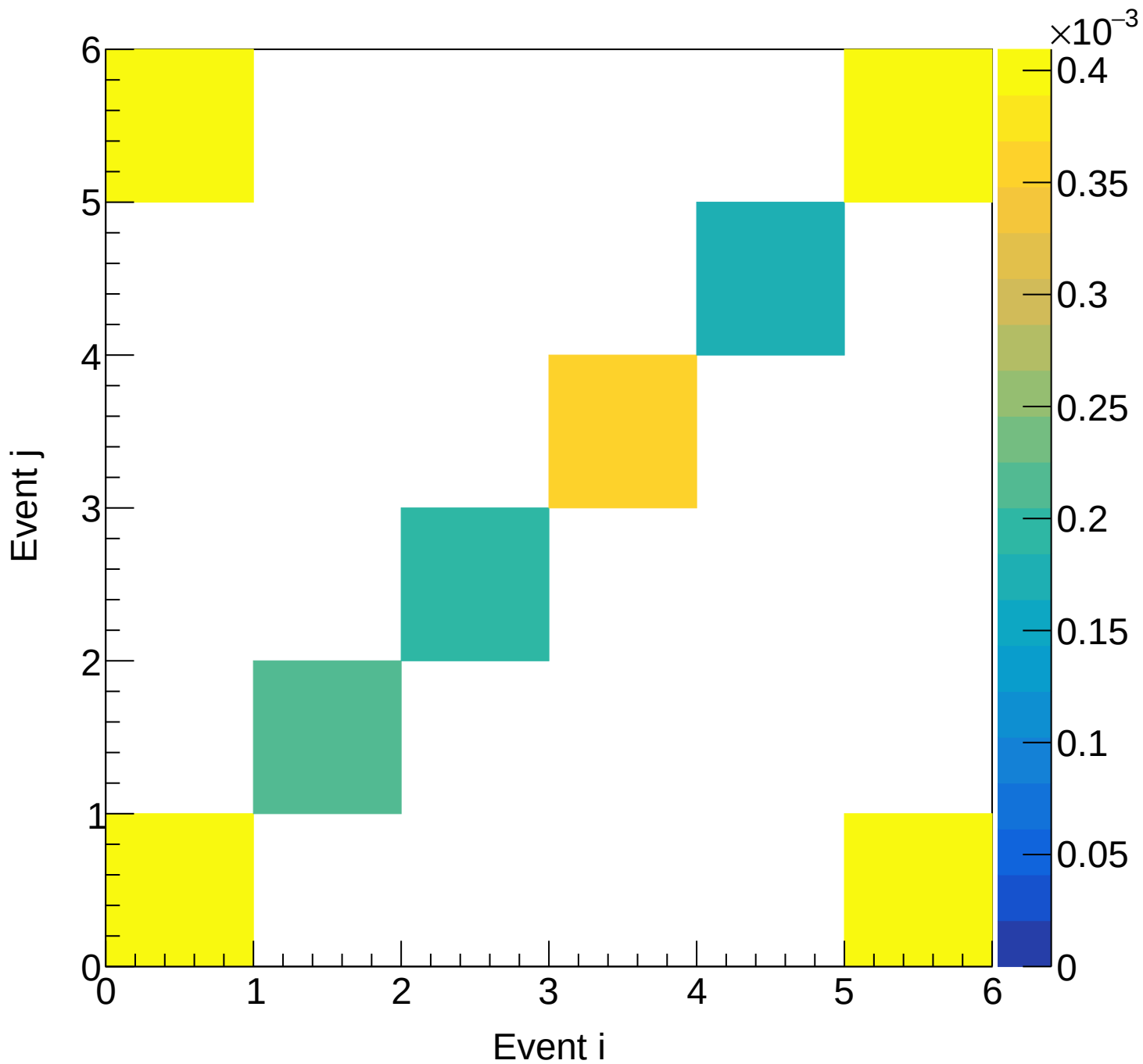
LD2 (total) Covariance | M: [4.8, 5.1) xF: [0.90, 0.95)
