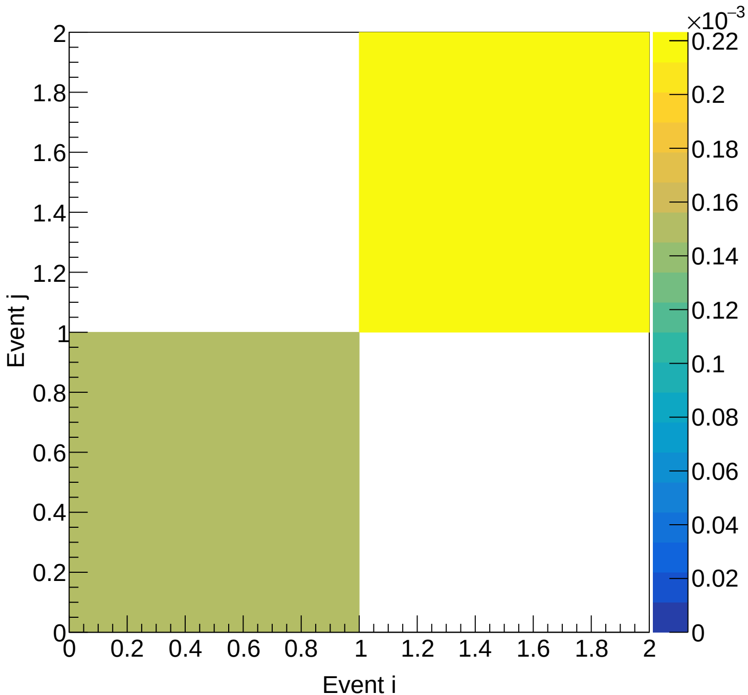
LD2 (total) Covariance | M: [5.1, 5.4) xF: [0.90, 0.95)
