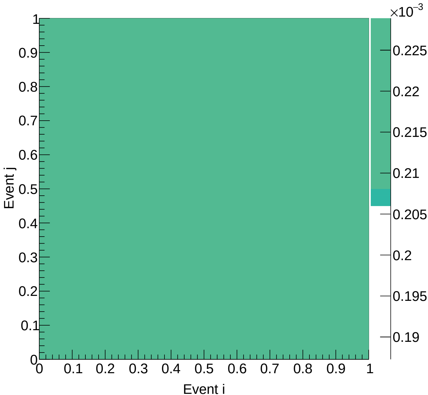
LD2 (total) Covariance | M: [4.2, 4.5) xF: [0.00, 0.05)
