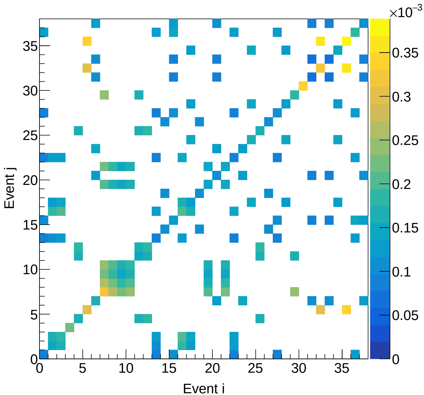
LD2 (total) Covariance | M: [4.8, 5.1) xF: [0.00, 0.05)
