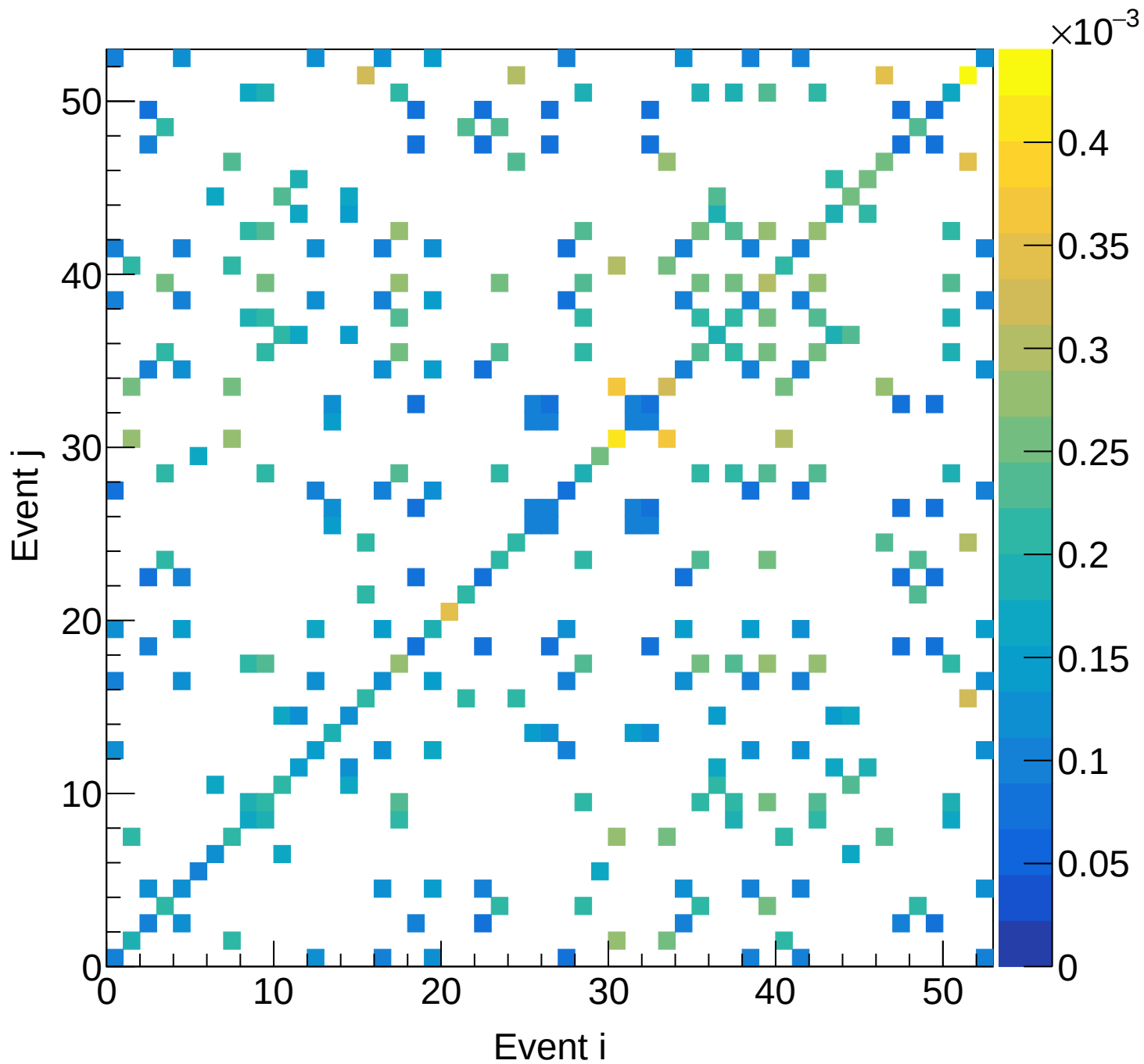
LD2 (total) Covariance | M: [5.4, 5.7] xF: [0.00, 0.05]
