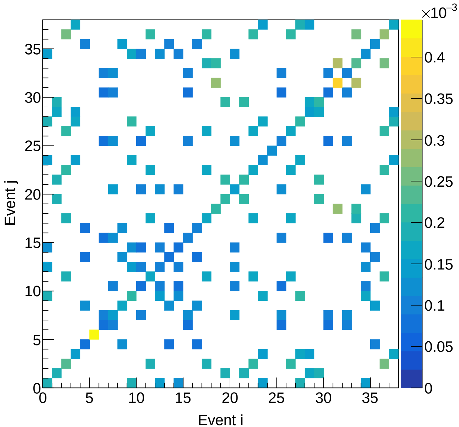
LD2 (total) Covariance | M: [5.7, 6.0] xF: [0.00, 0.05]
