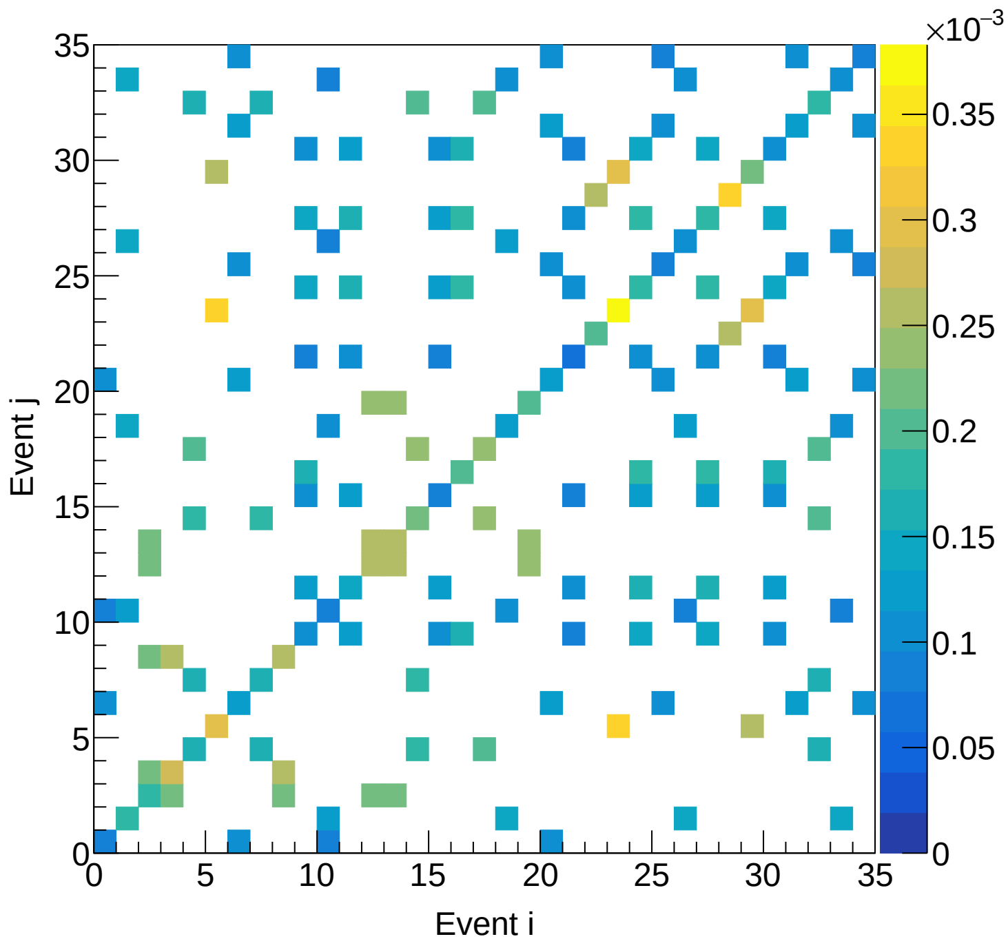
LD2 (total) Covariance | M: [6.0, 6.3] xF: [0.00, 0.05]
