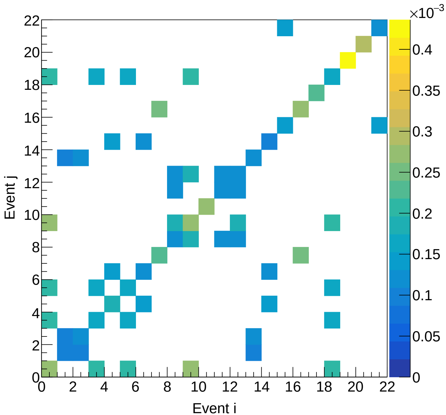
LD2 (total) Covariance | M: [6.3, 6.6] xF: [0.00, 0.05]
