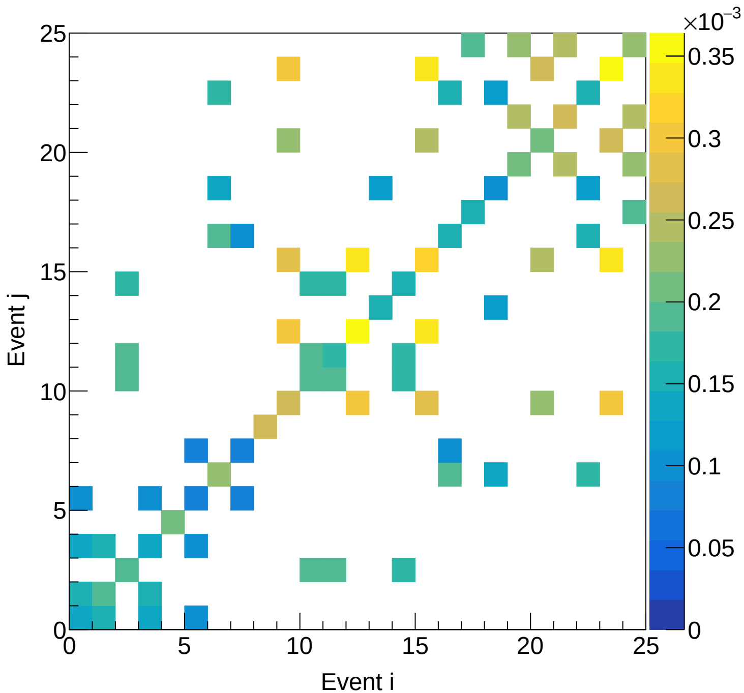
LD2 (total) Covariance | M: [4.5, 4.8) xF: [0.05, 0.10)
