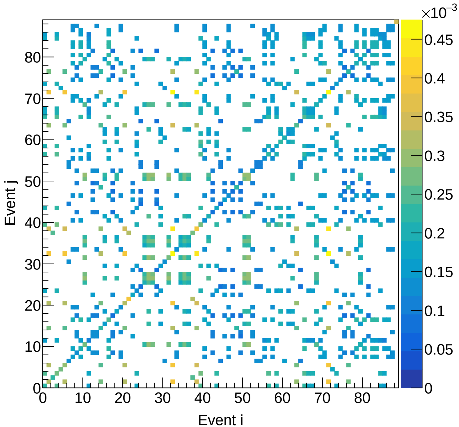
LD2 (total) Covariance | M: [5.1, 5.4) xF: [0.05, 0.10)
