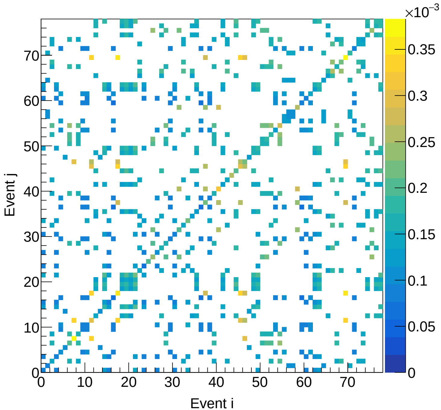
LD2 (total) Covariance | M: [5.4, 5.7) xF: [0.05, 0.10)
