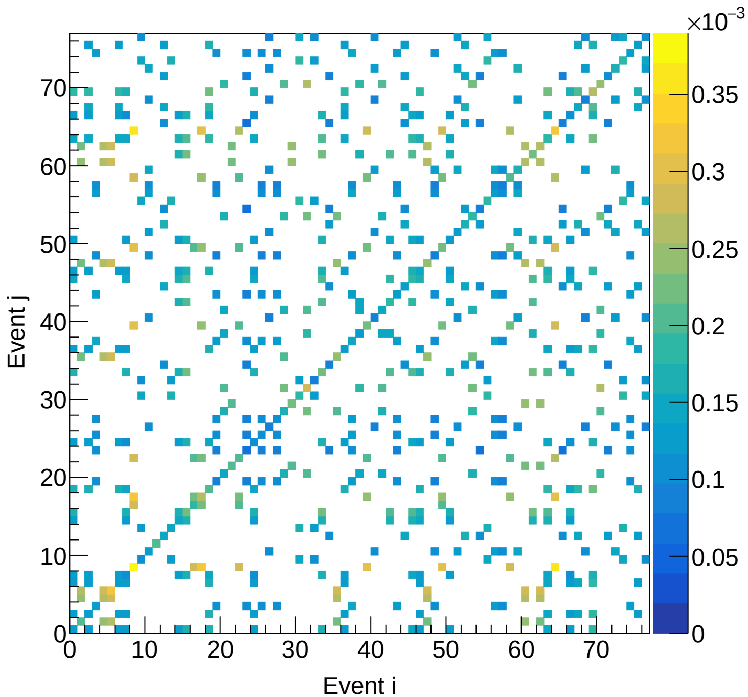
LD2 (total) Covariance | M: [5.7, 6.0] xF: [0.05, 0.10)
