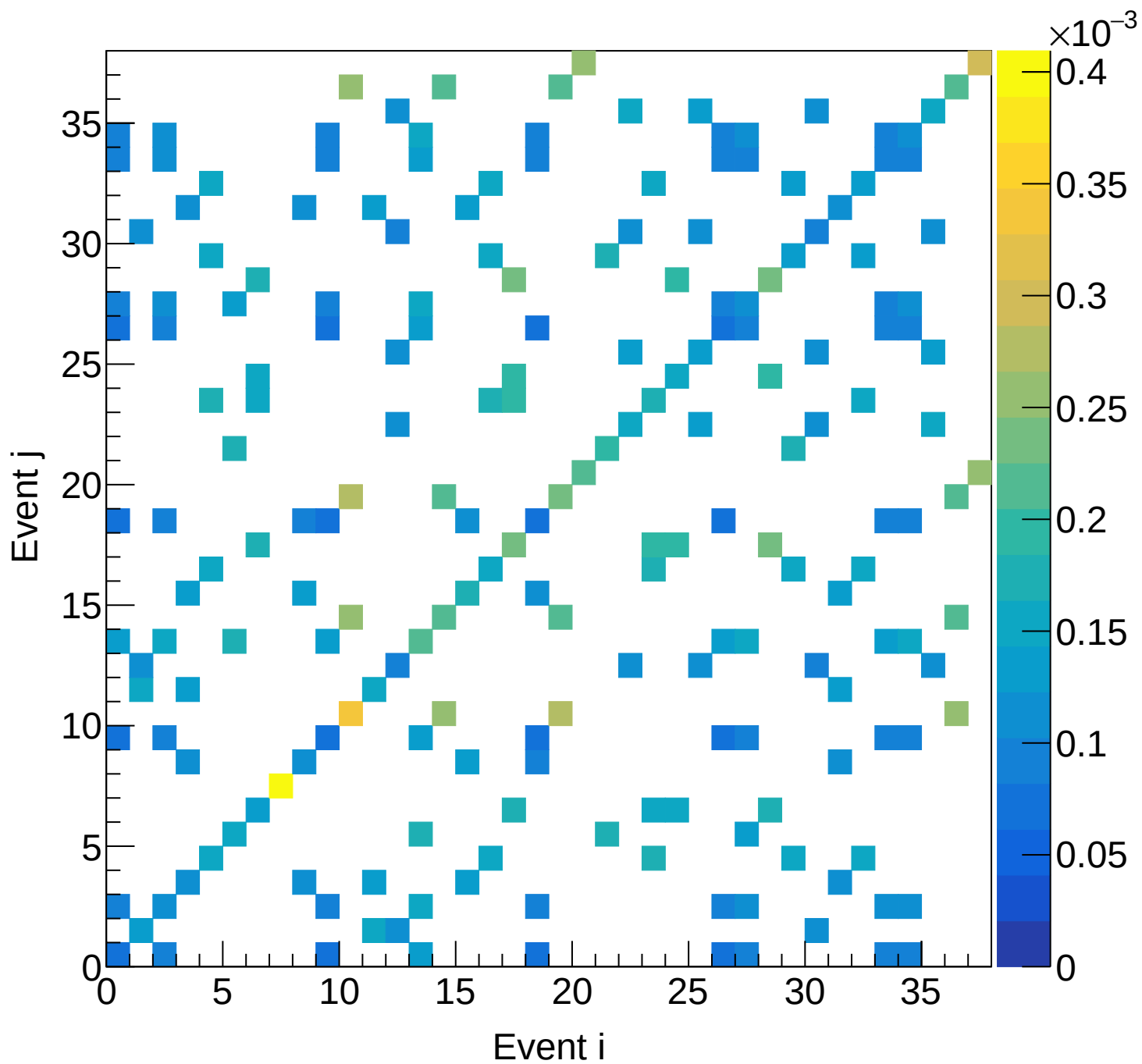
LD2 (total) Covariance | M: [6.0, 6.3] xF: [0.05, 0.10)
