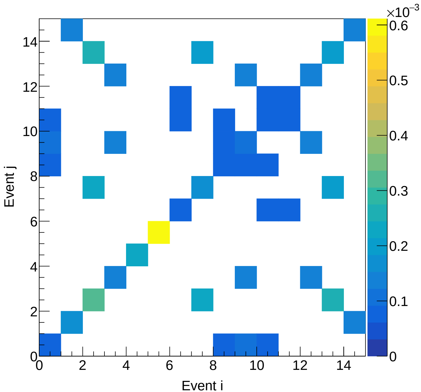
LD2 (total) Covariance | M: [6.6, 6.9) xF: [0.05, 0.10)
