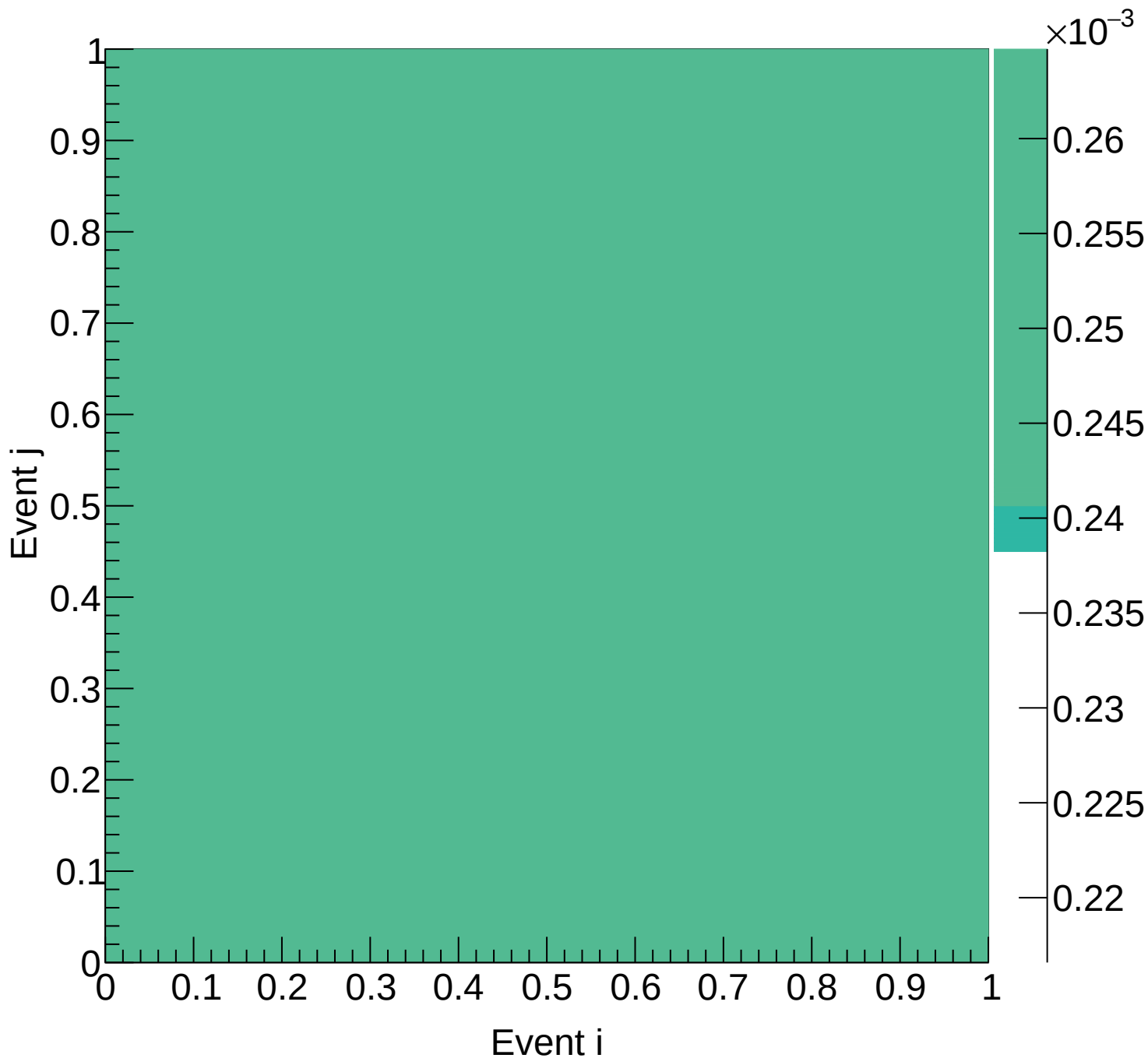
LD2 (total) Covariance | M: [7.5, 8.8) xF: [0.10, 0.15)
