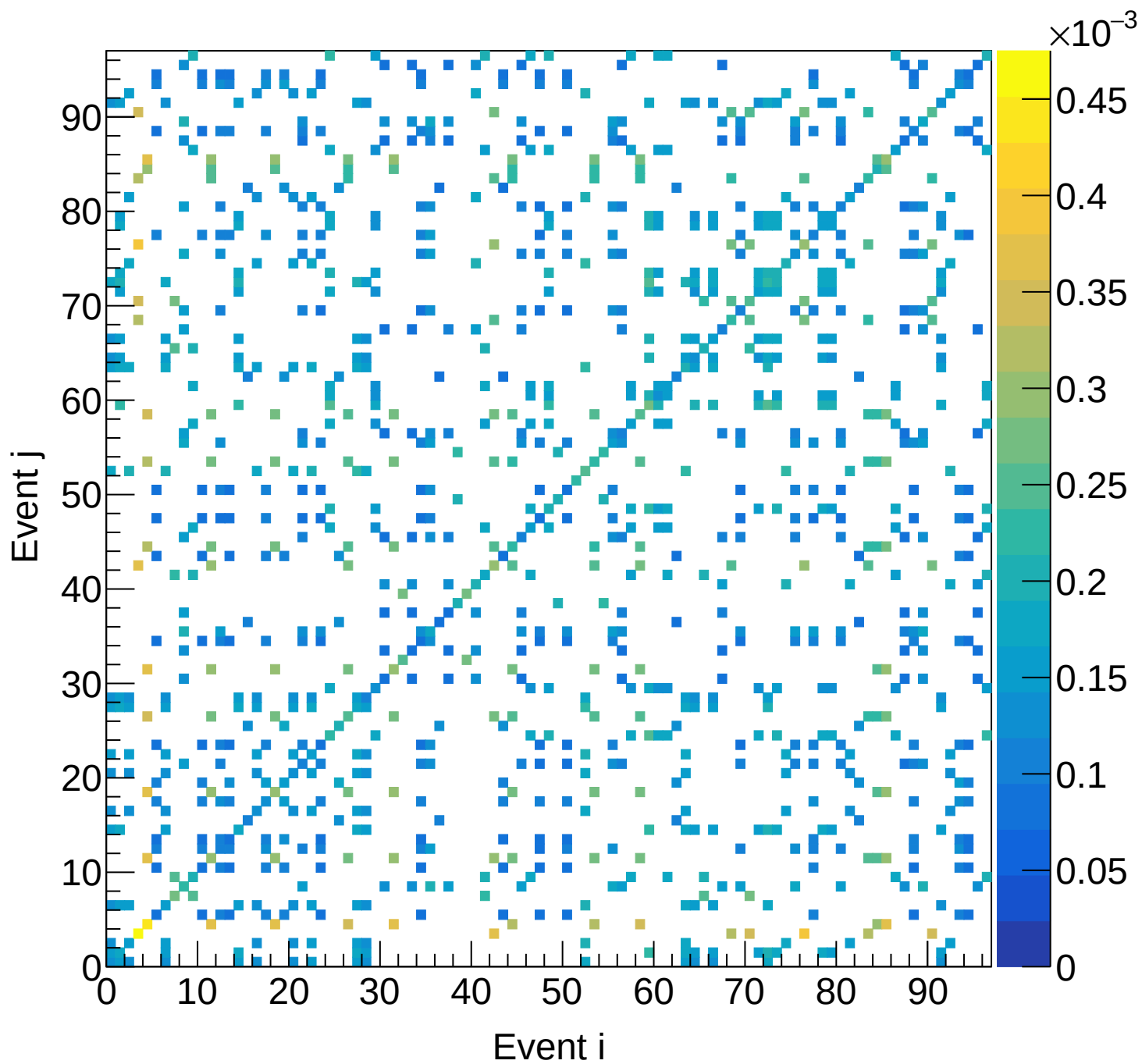
LD2 (total) Covariance | M: [4.5, 4.8) xF: [0.10, 0.15)
