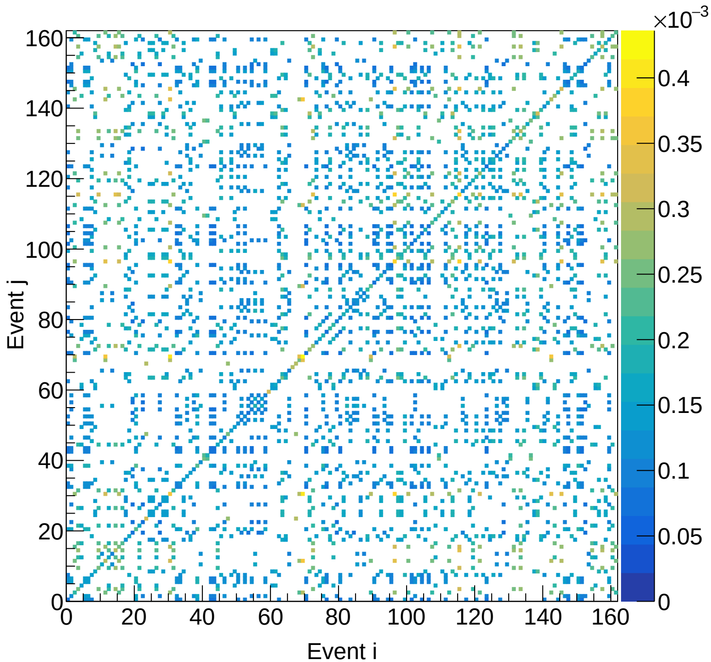
LD2 (total) Covariance | M: [4.8, 5.1) xF: [0.10, 0.15)
