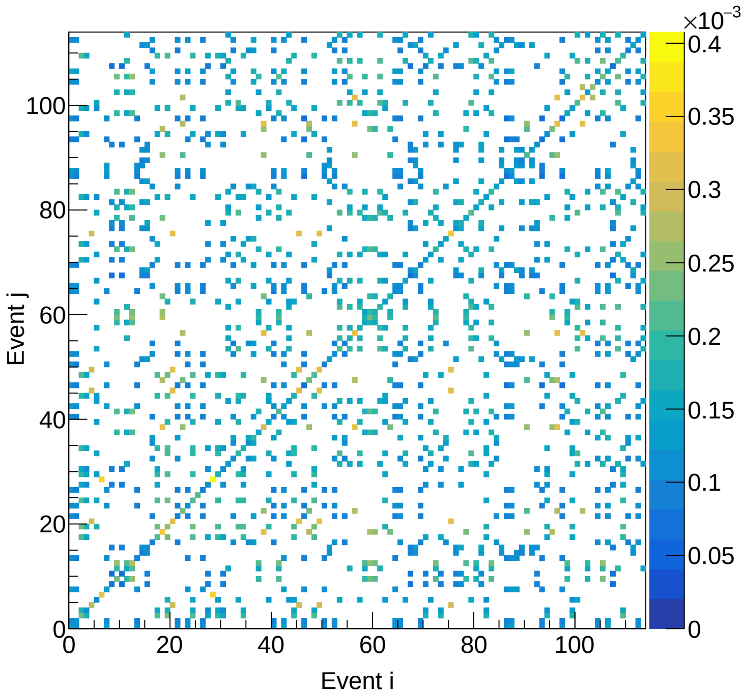
LD2 (total) Covariance | M: [5.4, 5.7) xF: [0.10, 0.15)
