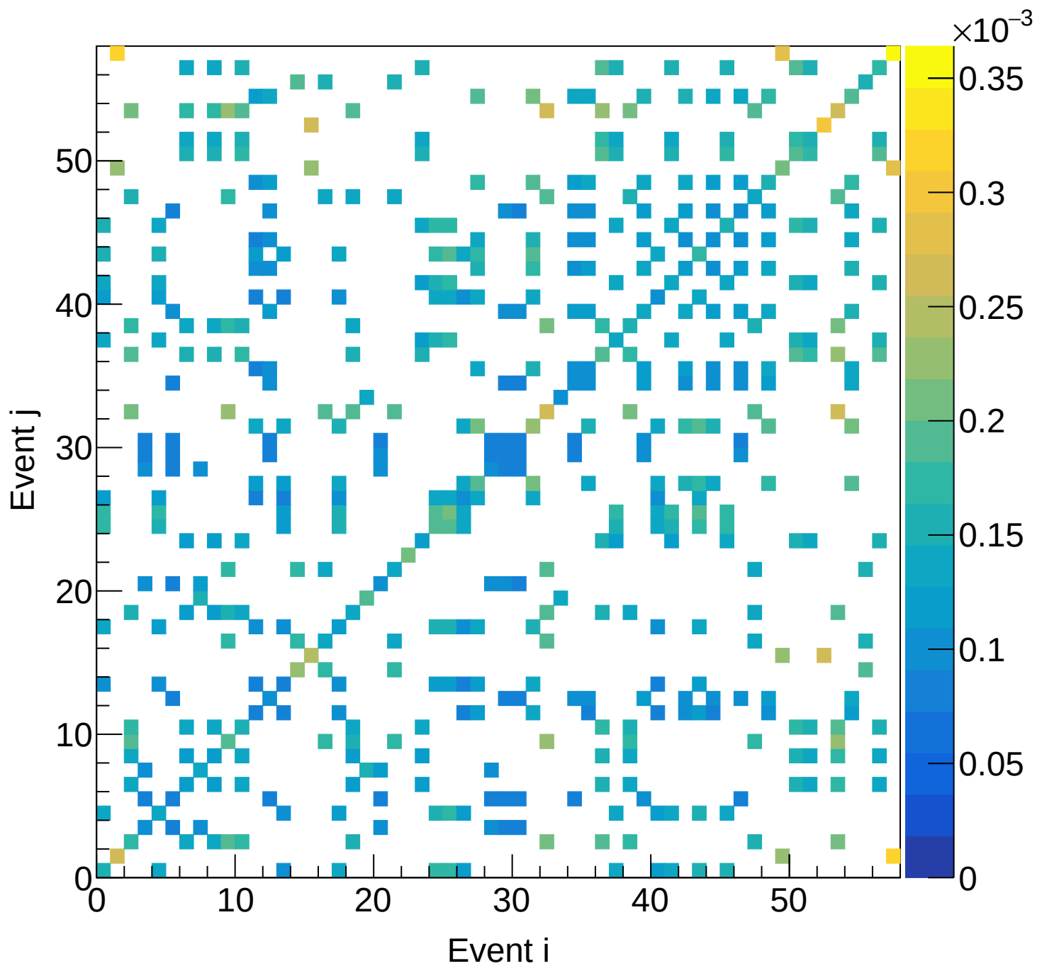
LD2 (total) Covariance | M: [6.0, 6.3) xF: [0.10, 0.15)
