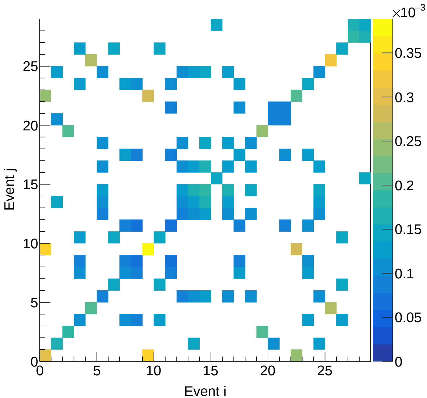
LD2 (total) Covariance | M: [6.3, 6.6) xF: [0.10, 0.15)
