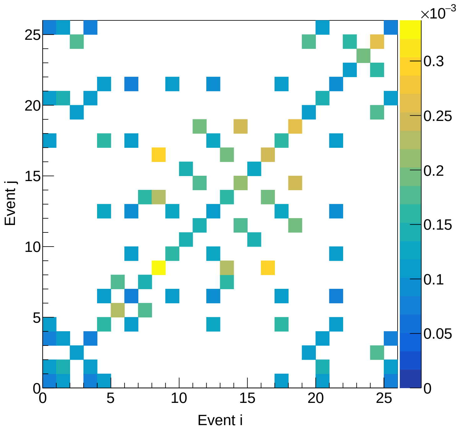
LD2 (total) Covariance | M: [6.6, 6.9) xF: [0.10, 0.15)
