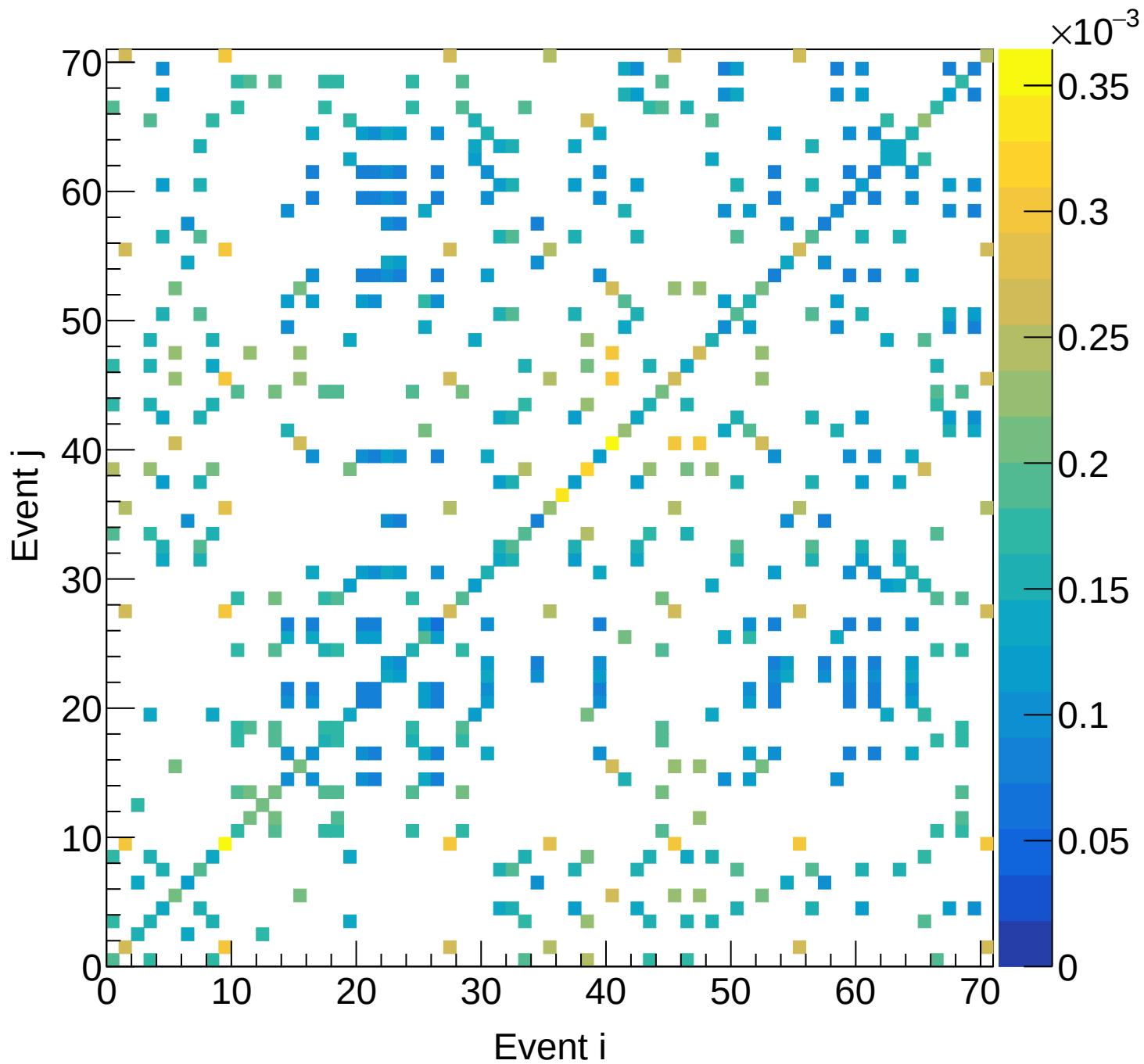
LD2 (total) Covariance | M: [4.2, 4.5) xF: [0.15, 0.20)
