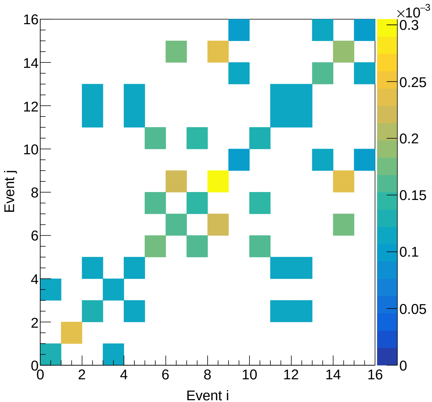
LD2 (total) Covariance | M: [6.9, 7.5) xF: [0.15, 0.20)
