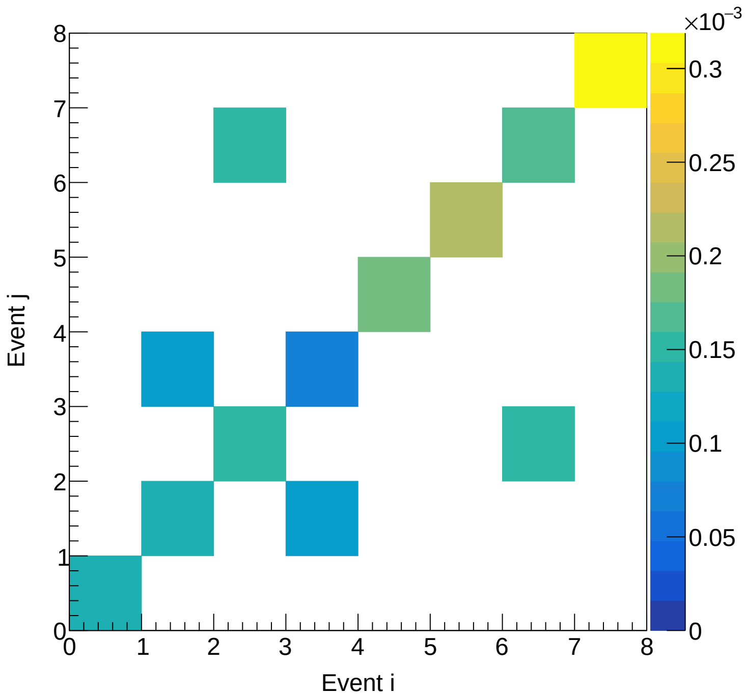
LD2 (total) Covariance | M: [7.5, 8.8) xF: [0.15, 0.20)
