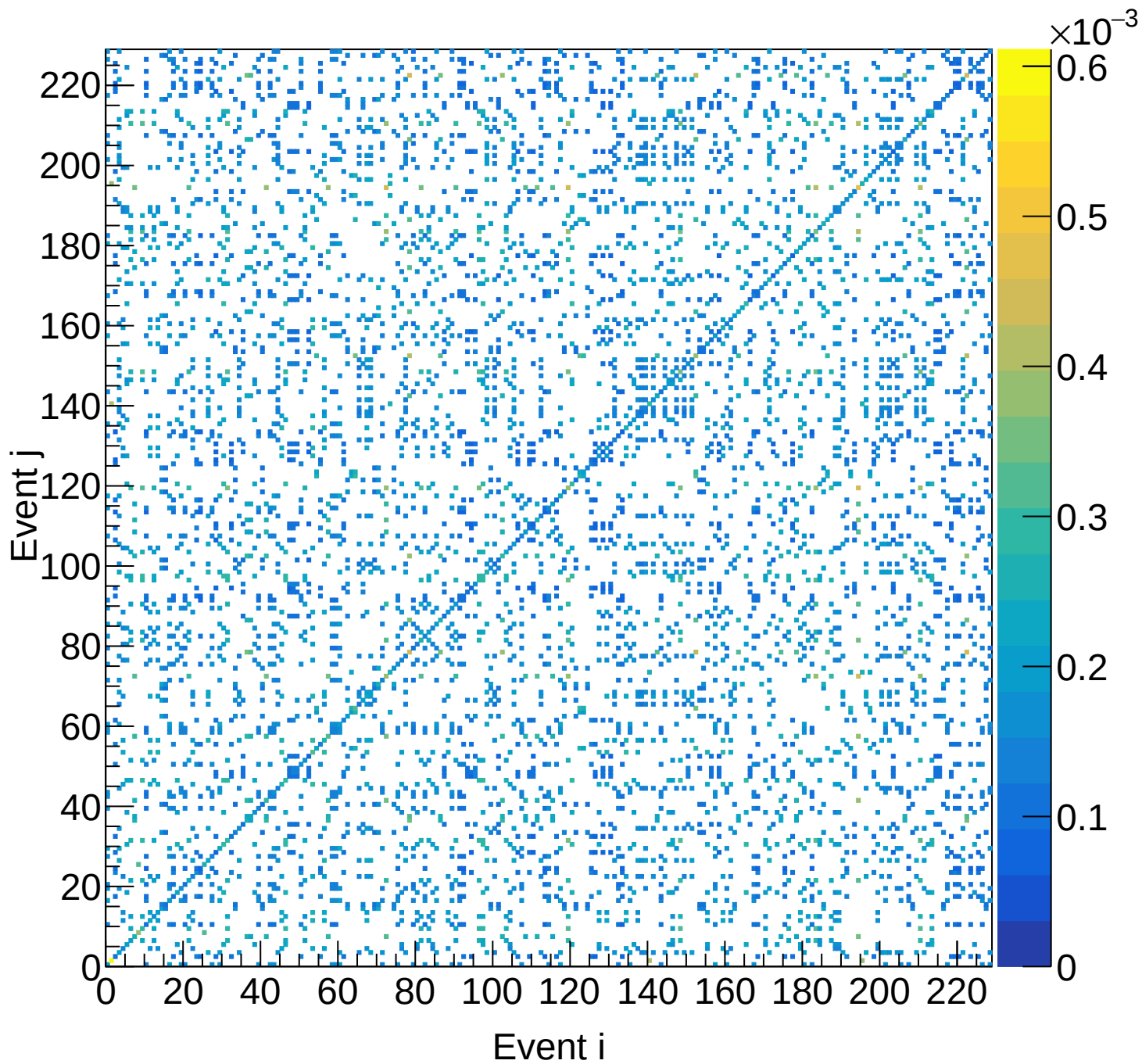
LD2 (total) Covariance | M: [4.8, 5.1) xF: [0.15, 0.20)
