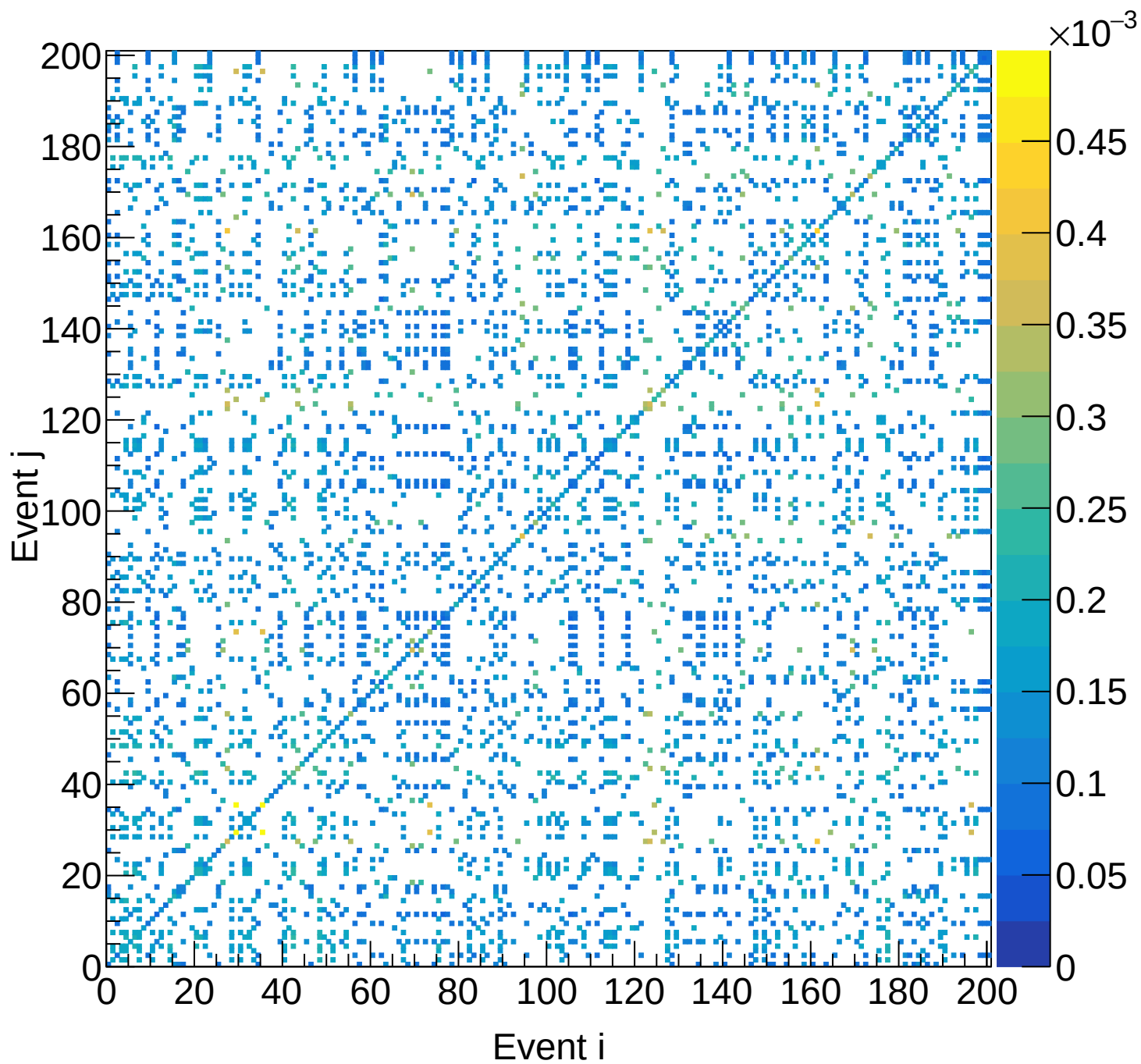
LD2 (total) Covariance | M: [5.1, 5.4) xF: [0.15, 0.20)
