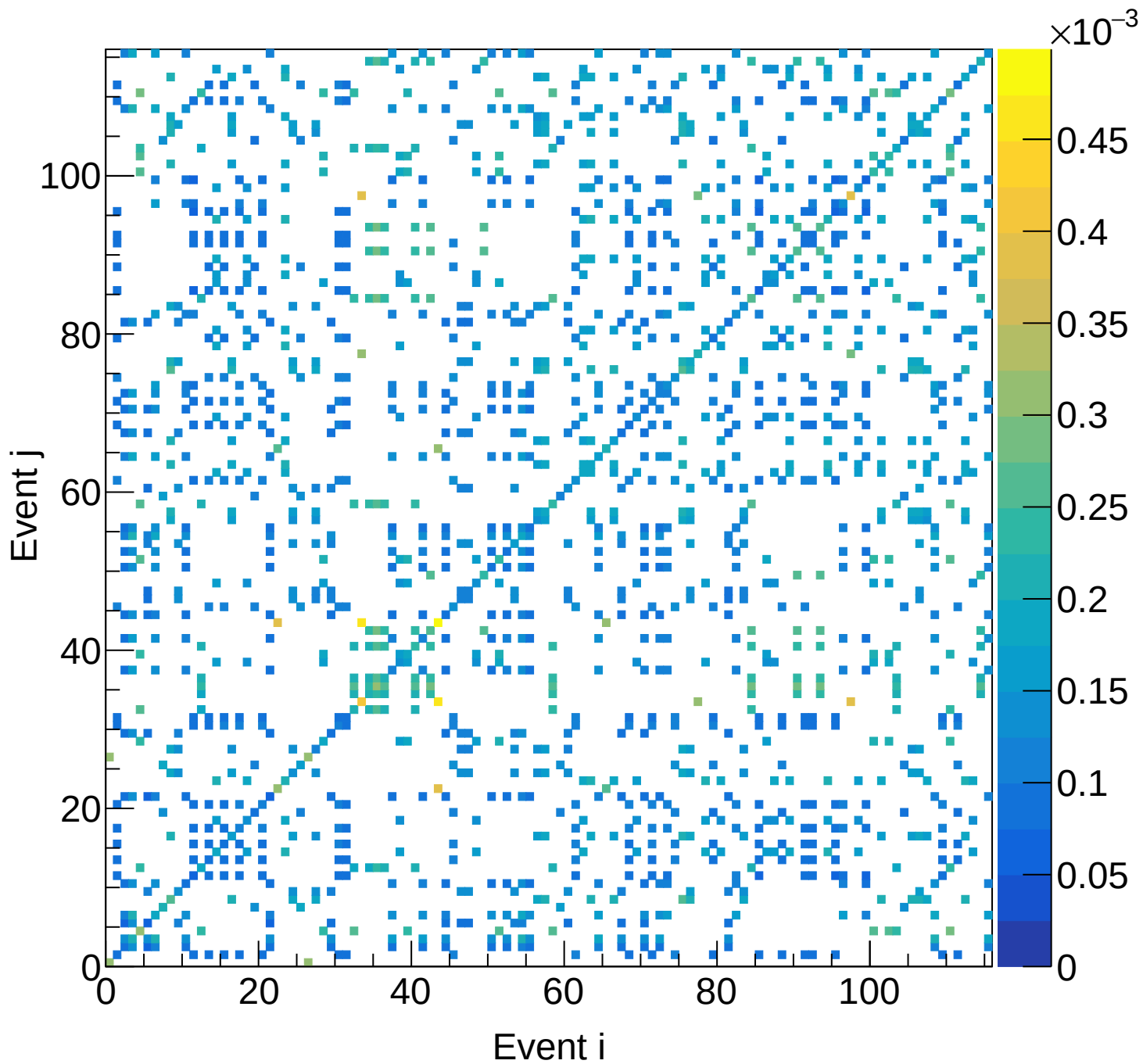
LD2 (total) Covariance | M: [5.7, 6.0) xF: [0.15, 0.20)
