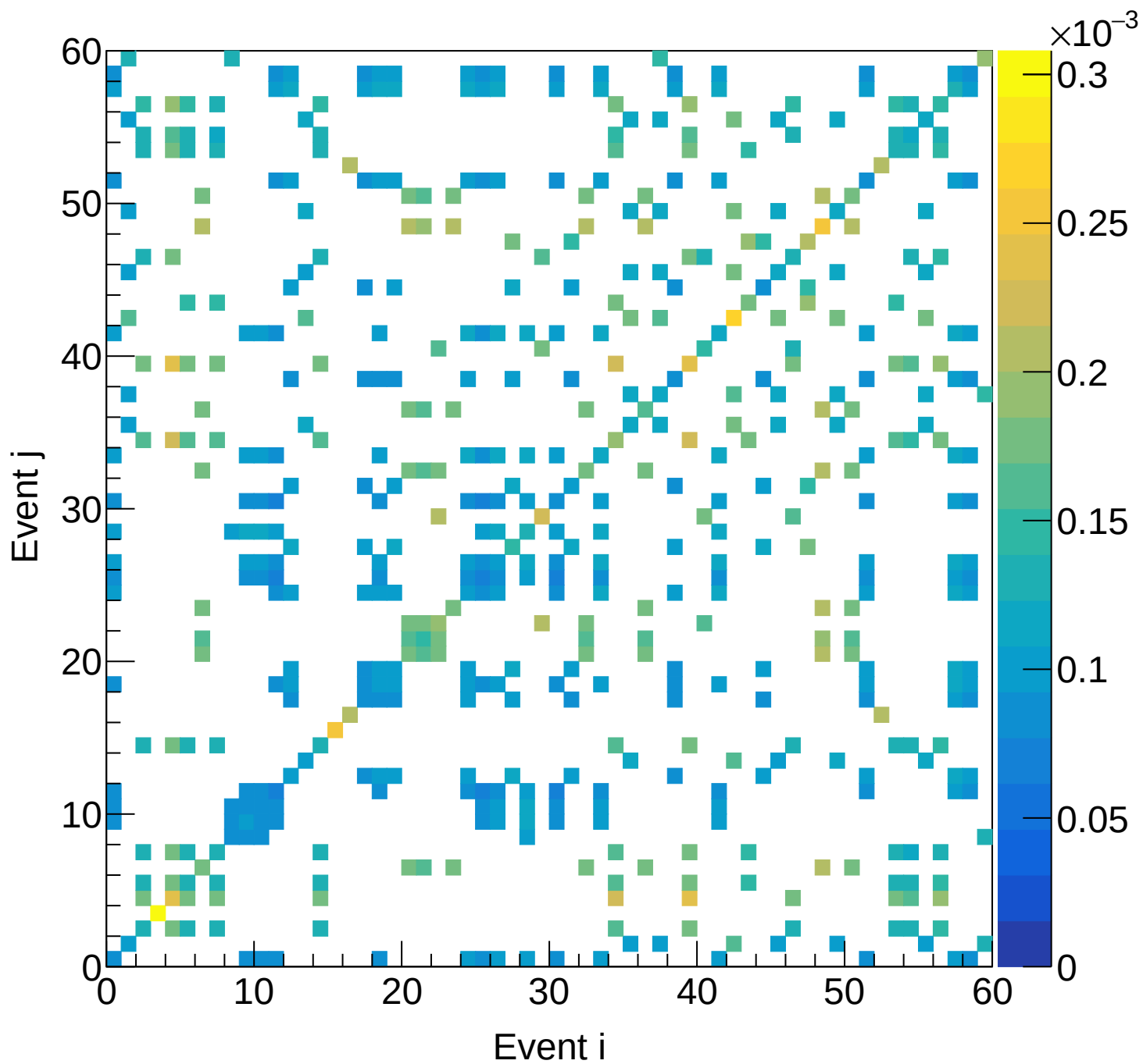
LD2 (total) Covariance | M: [6.0, 6.3) xF: [0.15, 0.20)
