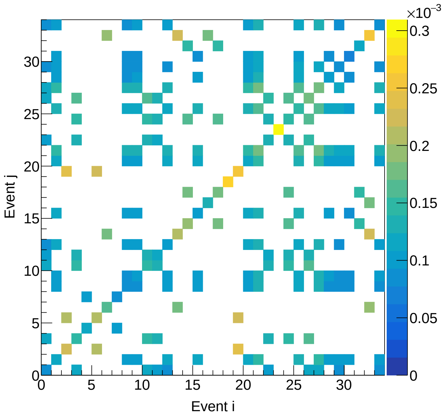
LD2 (total) Covariance | M: [6.3, 6.6) xF: [0.15, 0.20)
