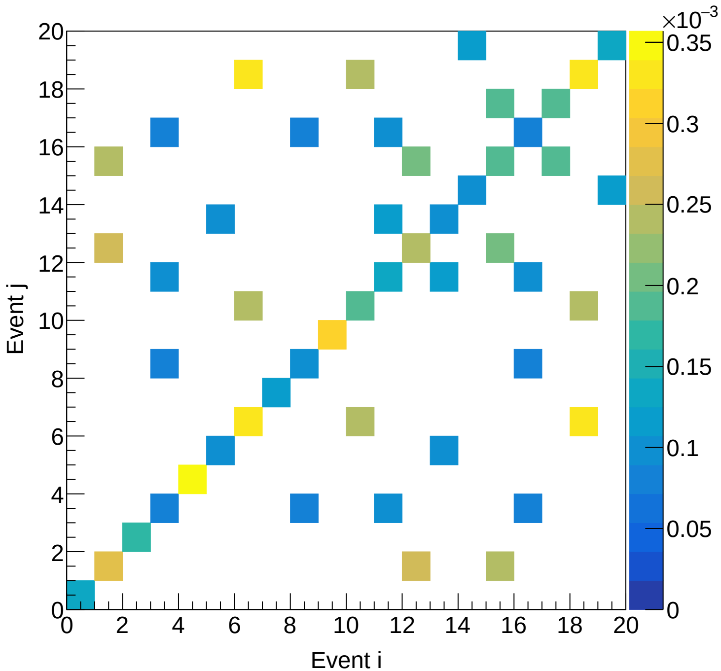
LD2 (total) Covariance | M: [6.6, 6.9] xF: [0.15, 0.20)
