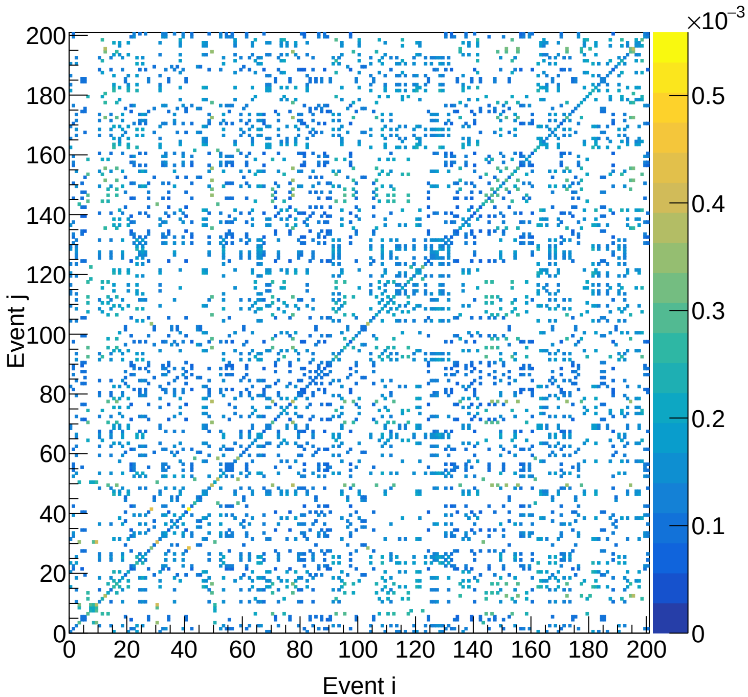
LD2 (total) Covariance | M: [4.2, 4.5) xF: [0.20, 0.25)
