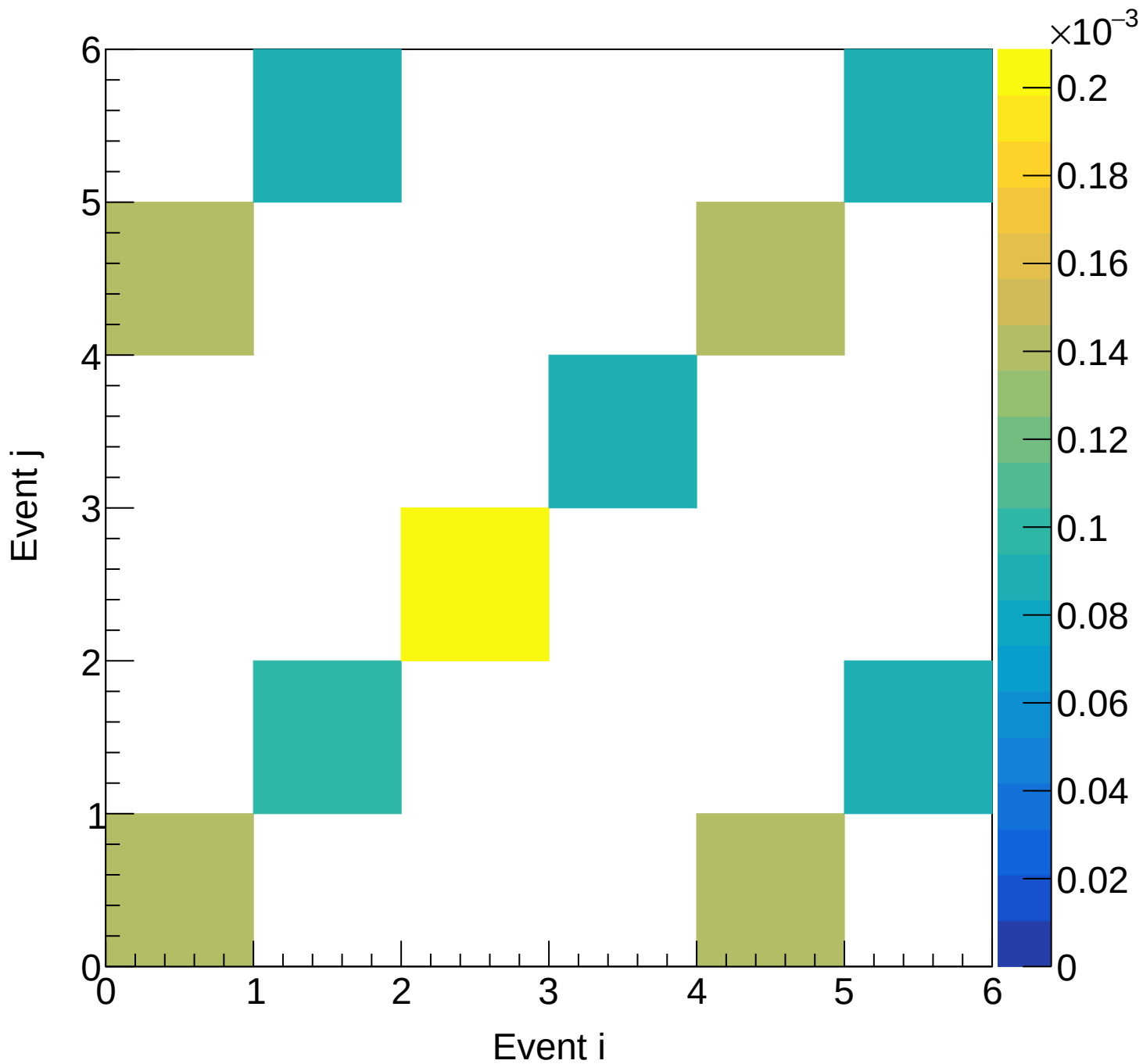
LD2 (total) Covariance | M: [7.5, 8.8) xF: [0.20, 0.25)
