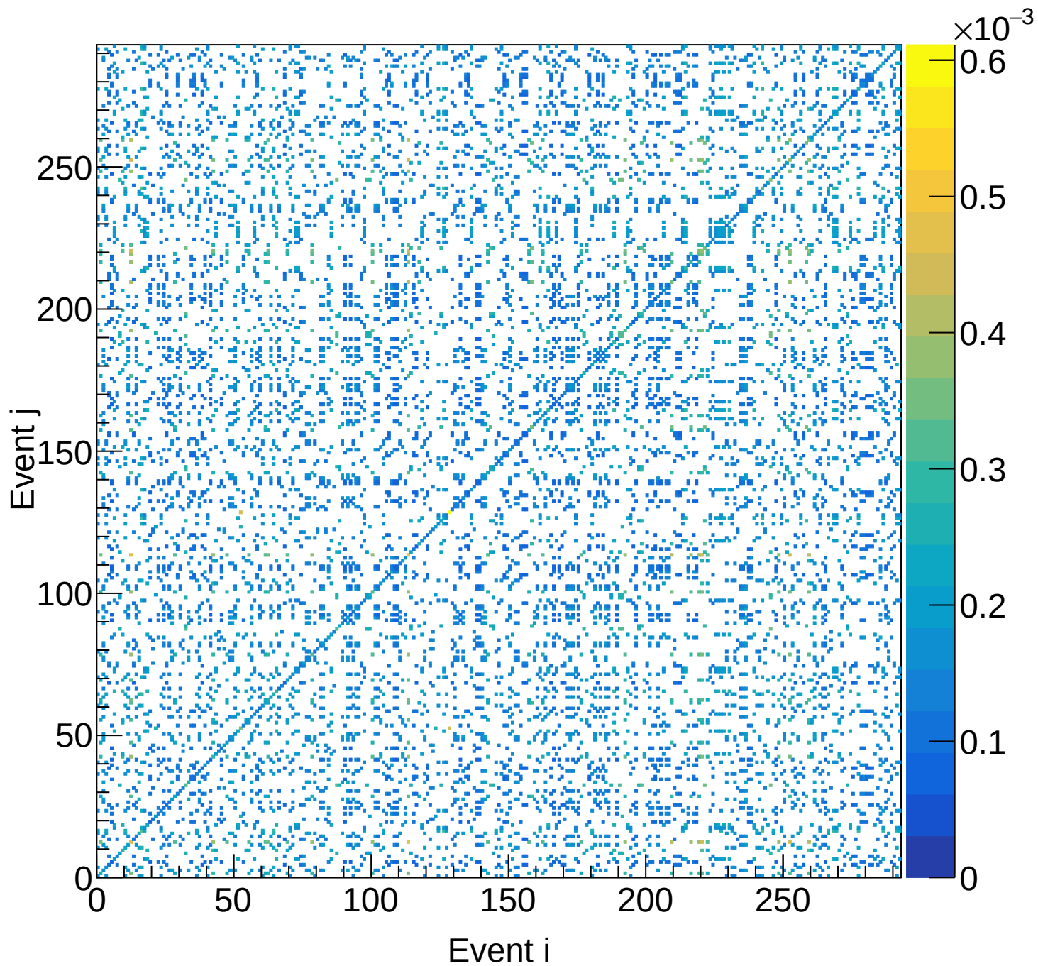
LD2 (total) Covariance | M: [4.5, 4.8) xF: [0.20, 0.25)
