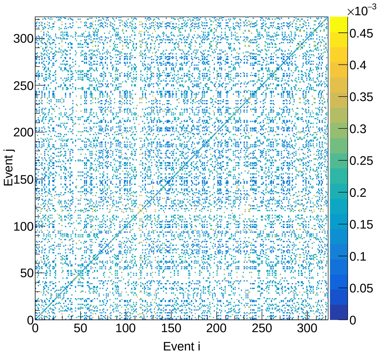
LD2 (total) Covariance | M: [4.8, 5.1) xF: [0.20, 0.25)
