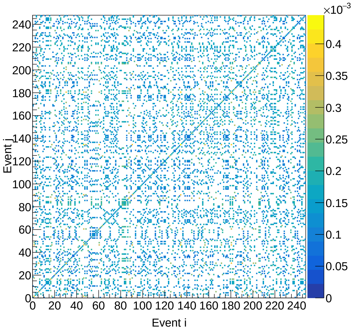
LD2 (total) Covariance | M: [5.1, 5.4) xF: [0.20, 0.25)
