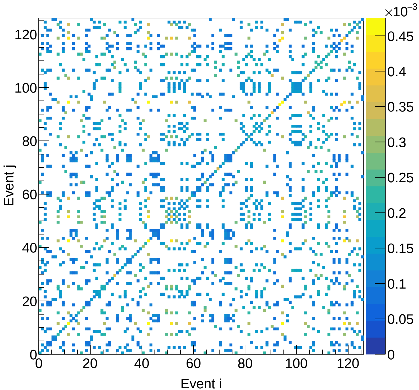
LD2 (total) Covariance | M: [5.7, 6.0) xF: [0.20, 0.25)
