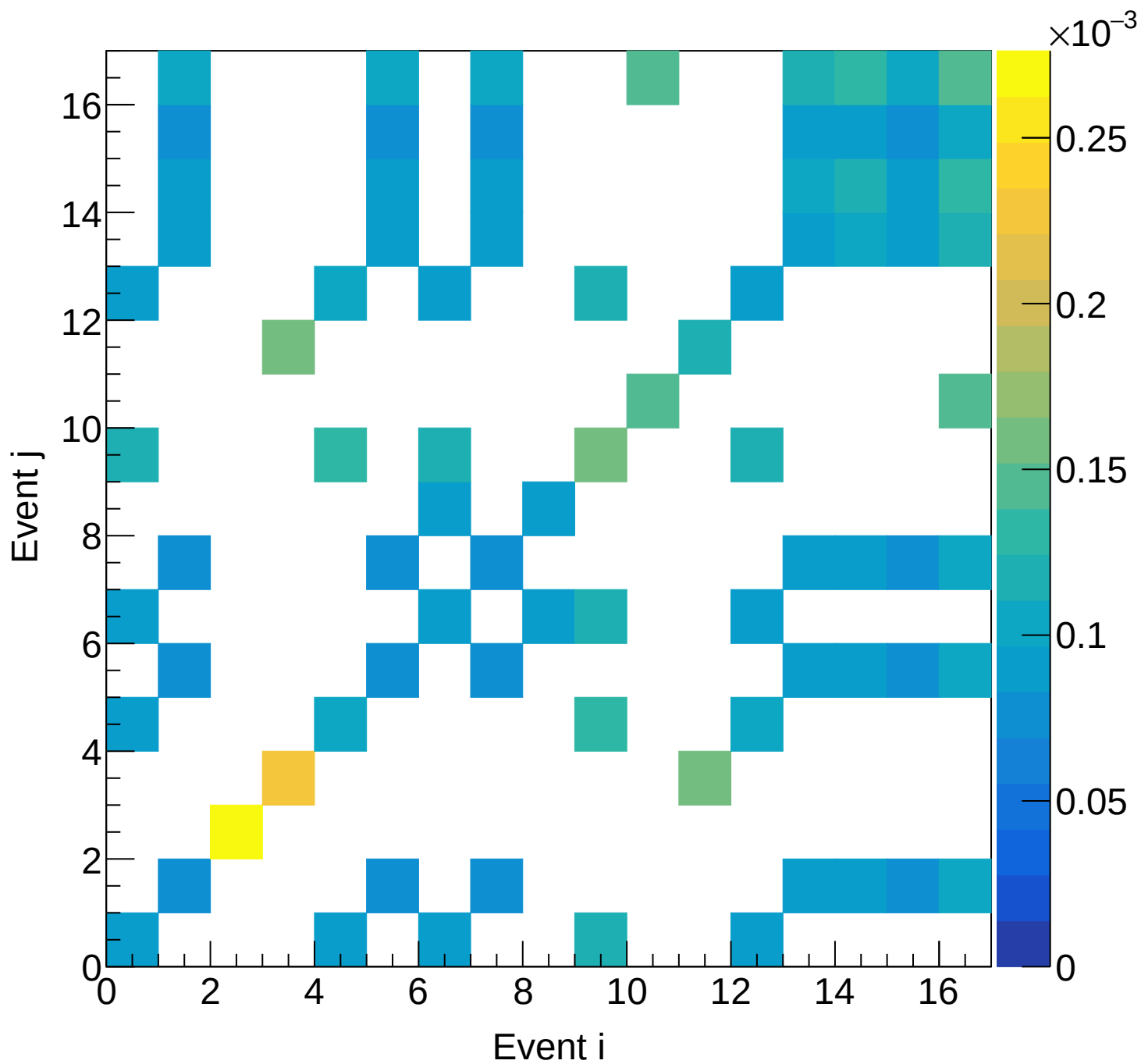
LD2 (total) Covariance | M: [6.6, 6.9) xF: [0.20, 0.25)
