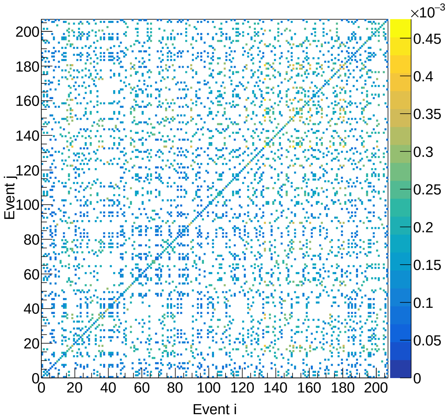
LD2 (total) Covariance | M: [3.9, 4.2) xF: [0.25, 0.30)
