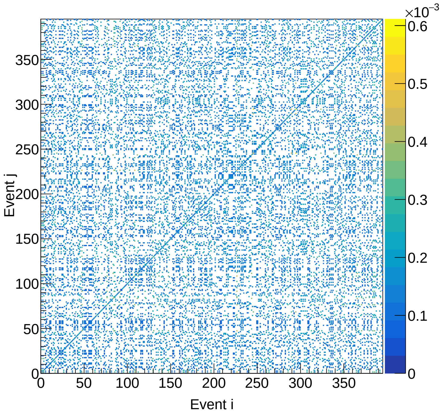
LD2 (total) Covariance | M: [4.2, 4.5) xF: [0.25, 0.30)
