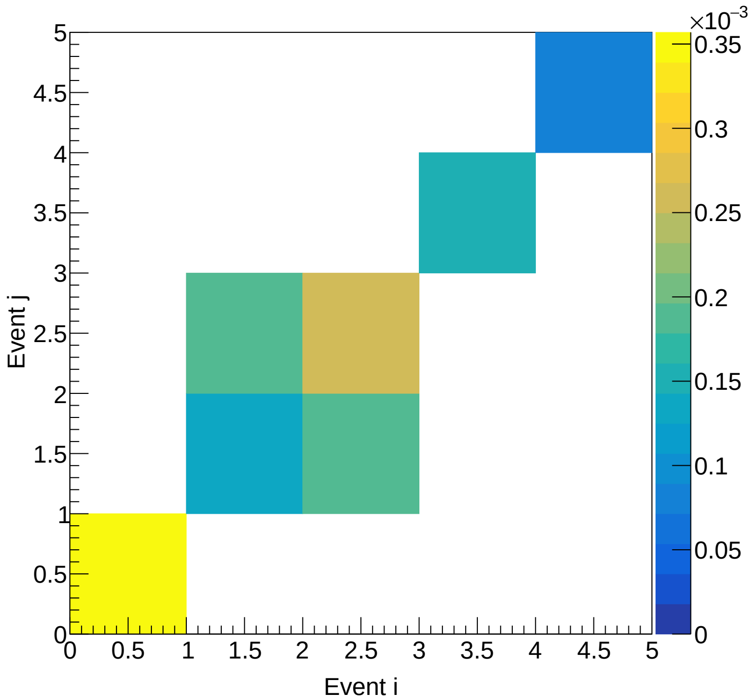
LD2 (total) Covariance | M: [7.5, 8.8) xF: [0.25, 0.30)
