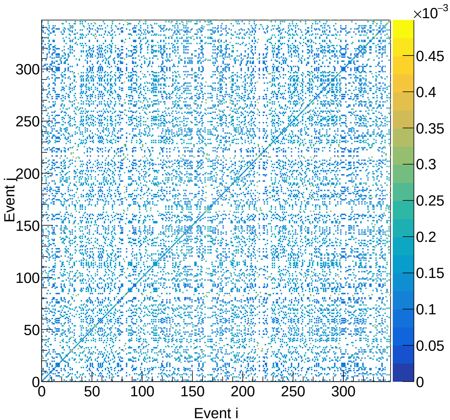
LD2 (total) Covariance | M: [4.8, 5.1) xF: [0.25, 0.30)
