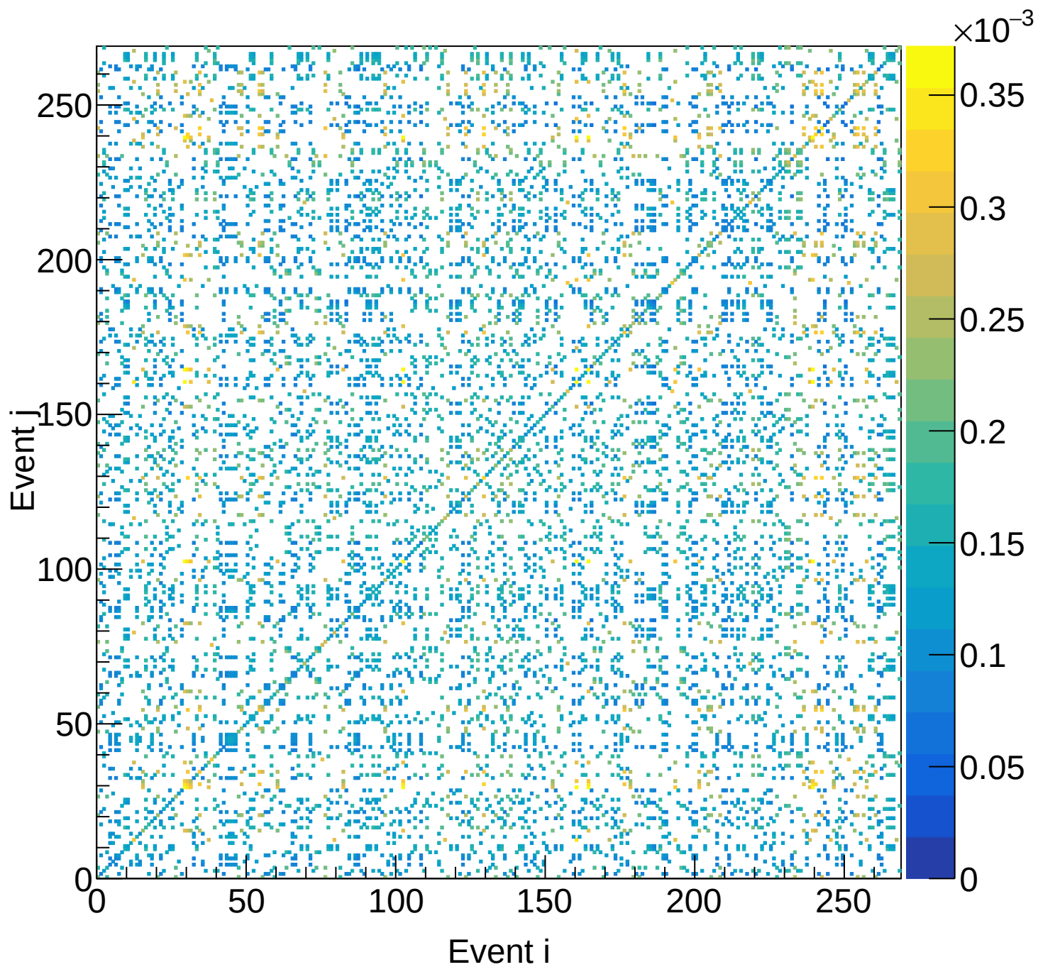
LD2 (total) Covariance | M: [5.1, 5.4) xF: [0.25, 0.30)
