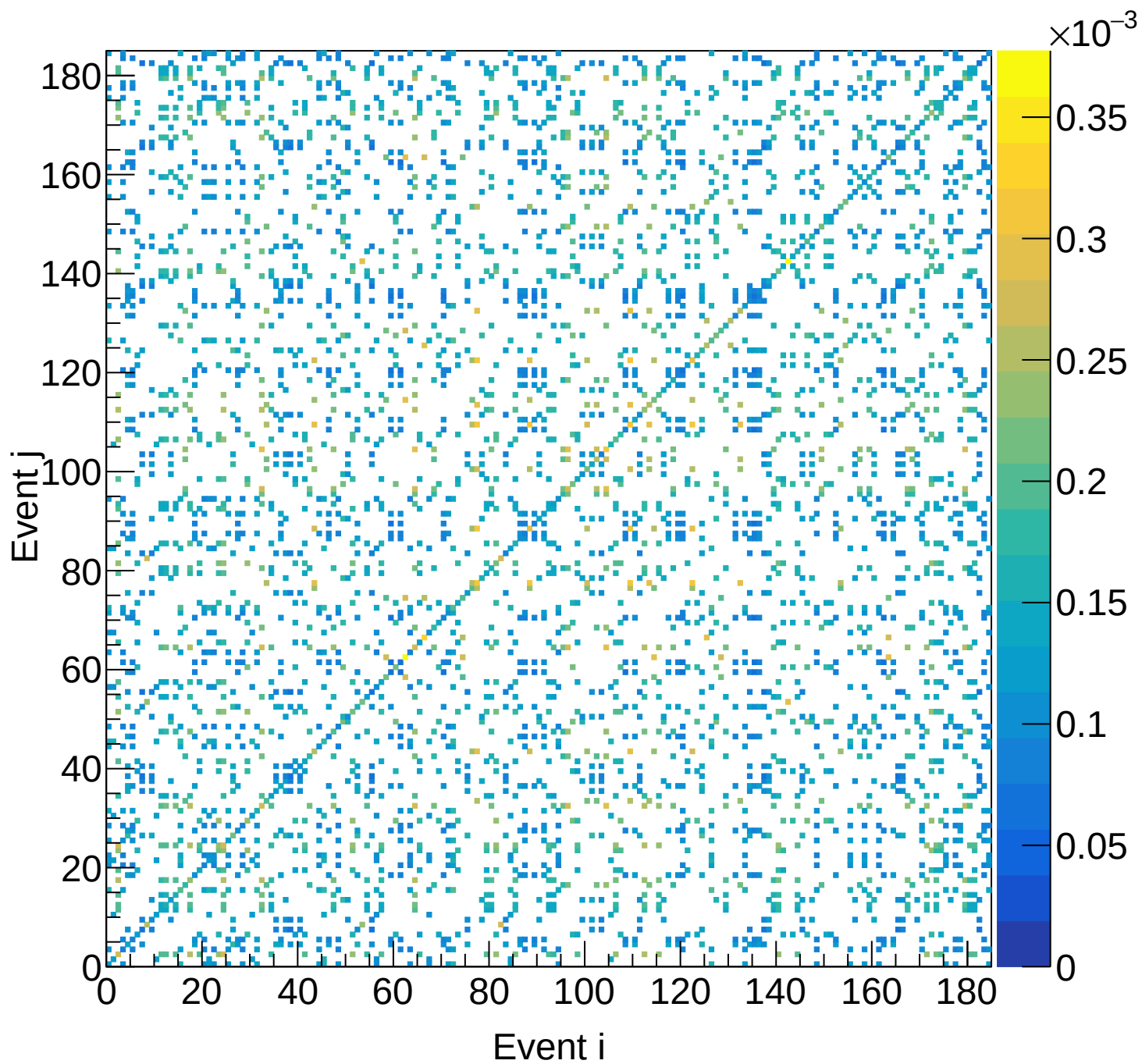
LD2 (total) Covariance | M: [5.4, 5.7) xF: [0.25, 0.30)
